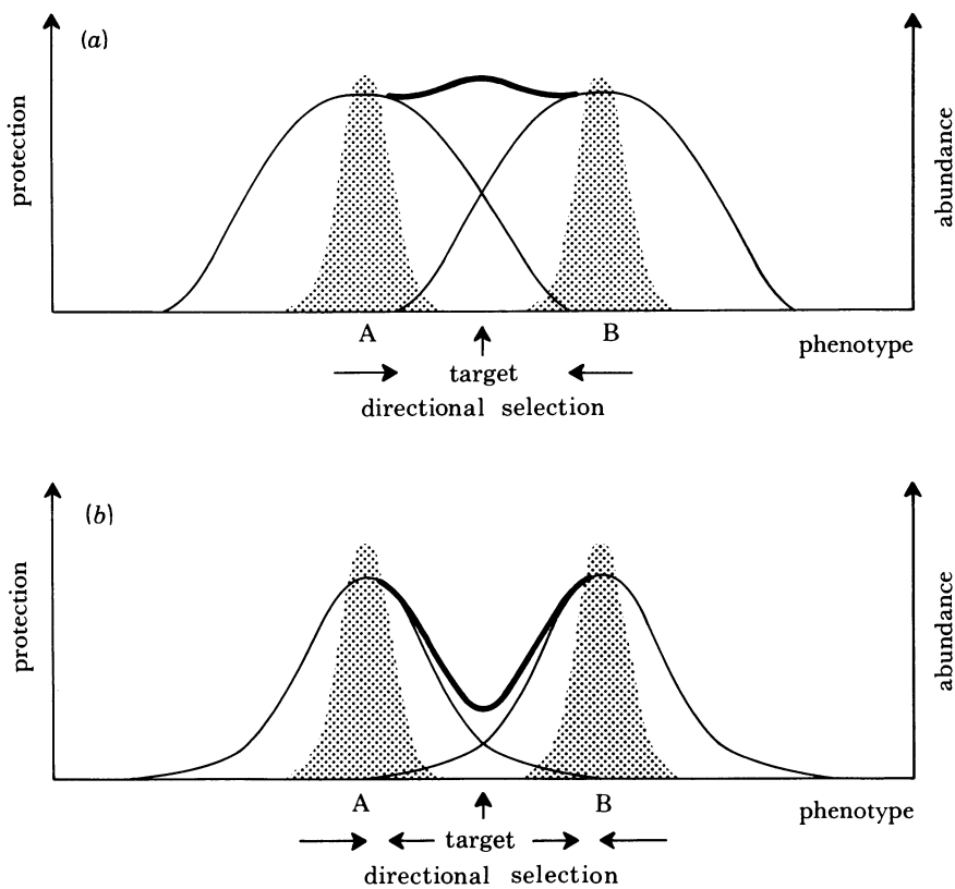
FIGURE 9. Gradual mutual convergence to a single 'target' phenotype of two warningly coloured species will occur when their curves of protection (thin lines) (assumed here to be equal) mutually overlap their phenotype distributions: any pattern occurring in the range of phenotypes between the two species is better protected (thick line) than it would be if only one of the species was present. The joint curve of protection (heavy line) might be convex (a) or concave (b) upward according to a variety of circumstances, but the target pattern will still be the same.
